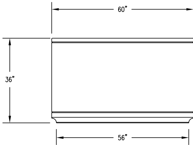
2 ELEVATION VIEW
