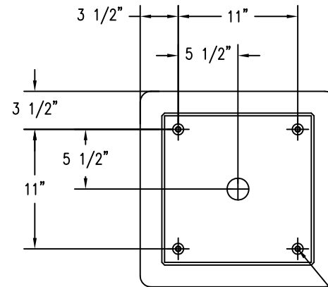
3 BOTTOM VIEW
