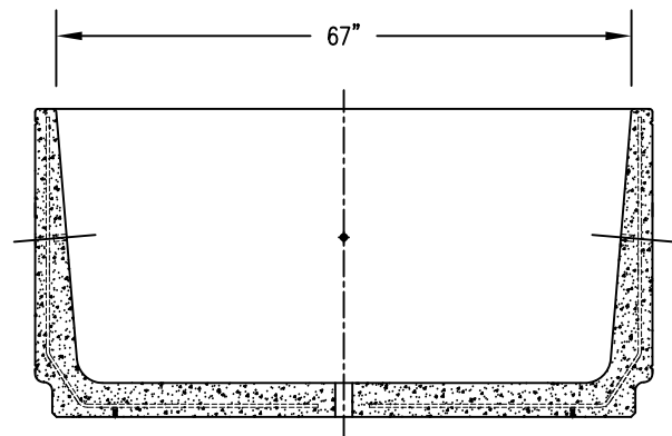
4 CROSS SECTION
