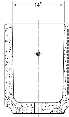
4 CROSS SECTION
