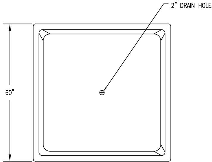
1 TOP VIEW
