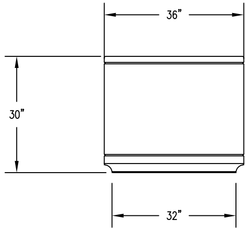
2 ELEVATION VIEW
