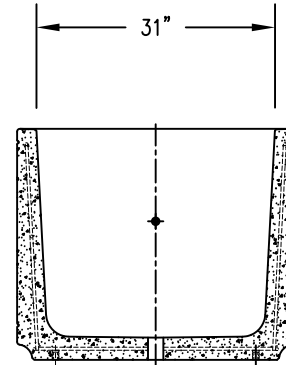
4 CROSS SECTION
