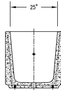
4 CROSS SECTION
