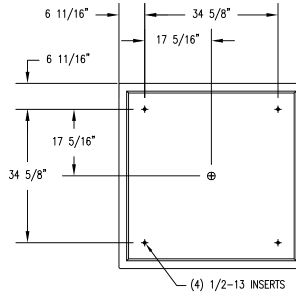
3 BOTTOM VIEW
