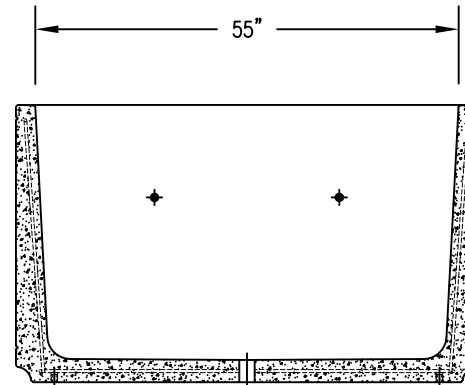
4 CROSS SECTION
