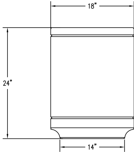
2 ELEVATION VIEW
