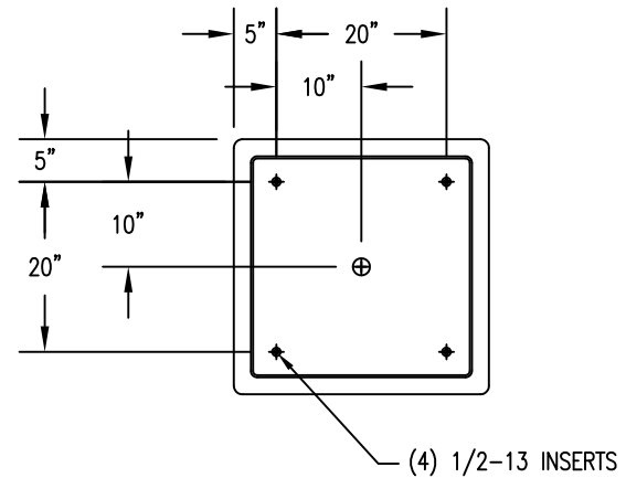
3 BOTTOM VIEW
