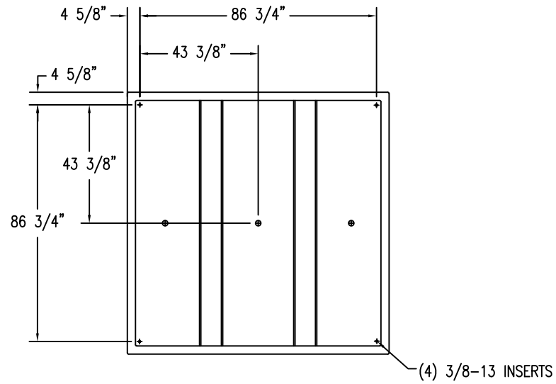
3 BOTTOM VIEW
