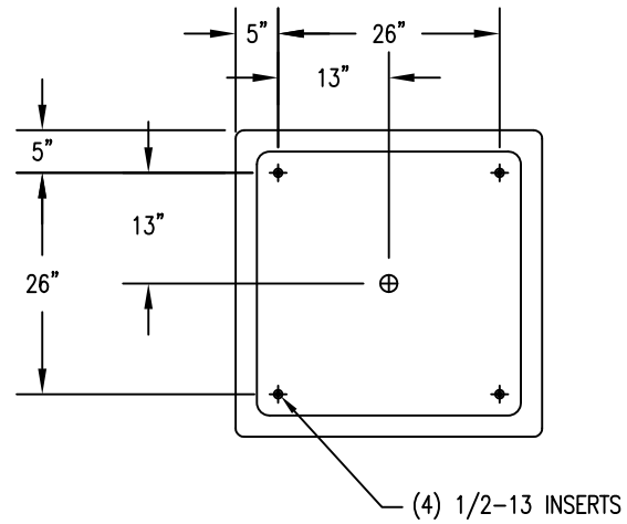
3 BOTTOM VIEW
