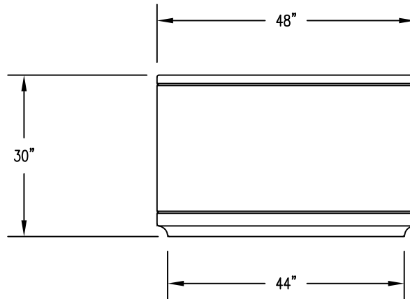
2 ELEVATION VIEW
