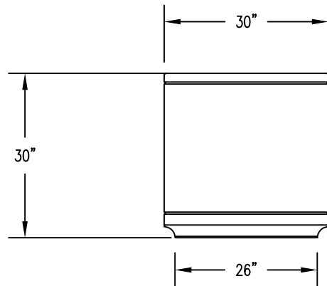
2 ELEVATION VIEW
