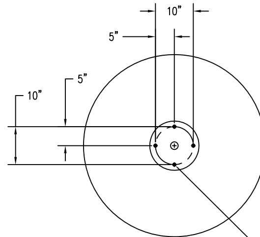
3 BOTTOM VIEW
