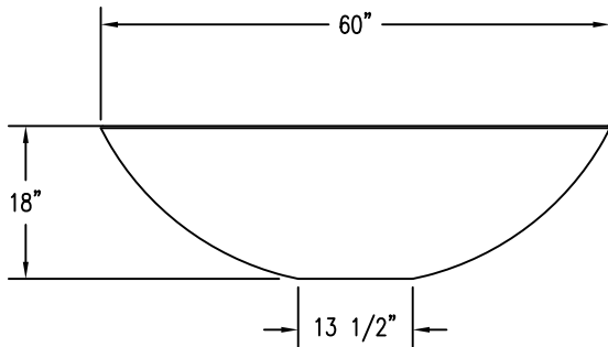
2 ELEVATION VIEW
