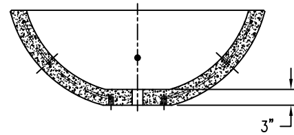
4 CROSS SECTION
