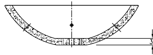
4 CROSS SECTION
