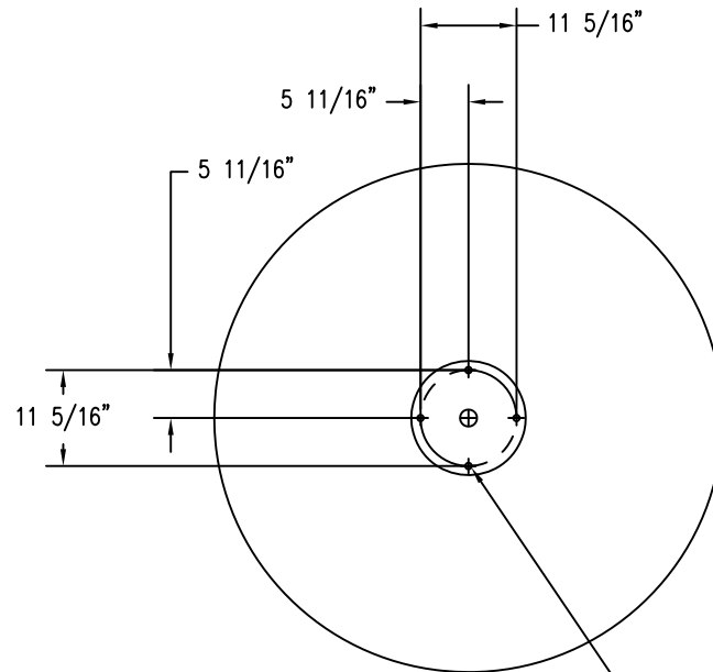
3 BOTTOM VIEW
